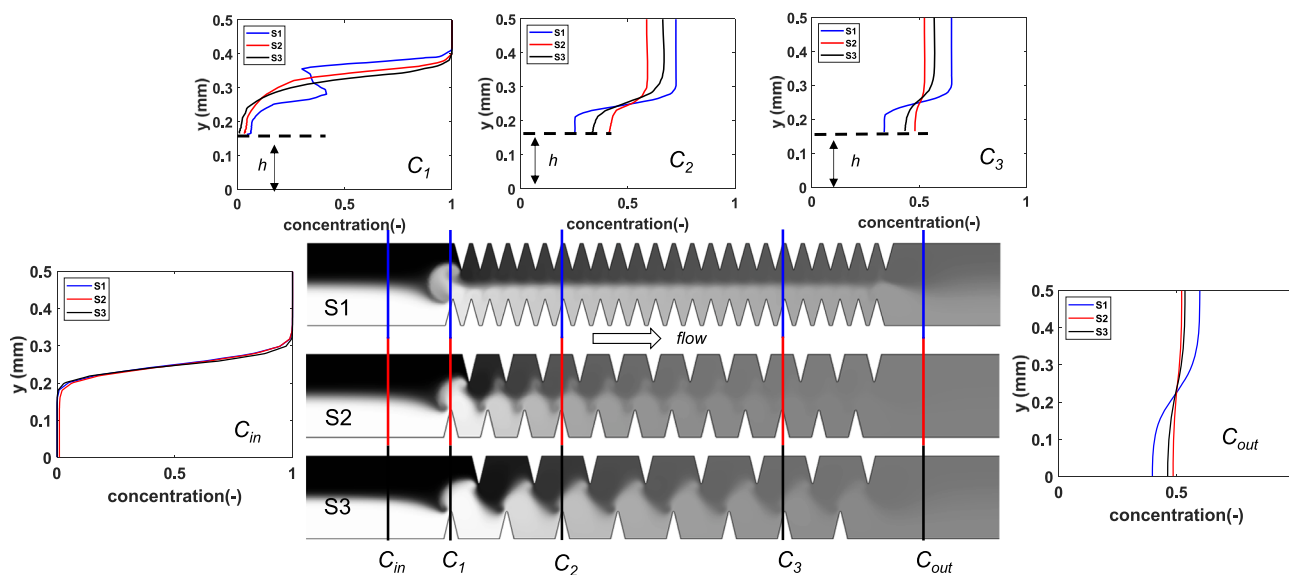
Fig. 6. Comparison of mixing performance of three micromixers S1/S2/S3. Concentration gray level maps from numerical simulation under the same following conditions: v_a=130 mm/s and Q_c= 8 \mu L/min. Cross-section concentration profiles are shown as inserts, for different longitudinal locations. Concentration curves from C_{in} to C_{out} quantitatively confirms the performance order from S2>S3>S1 , with an identical inlet condition C_{in} . Normalized concentration, from 0 to 1, is utilized here.
