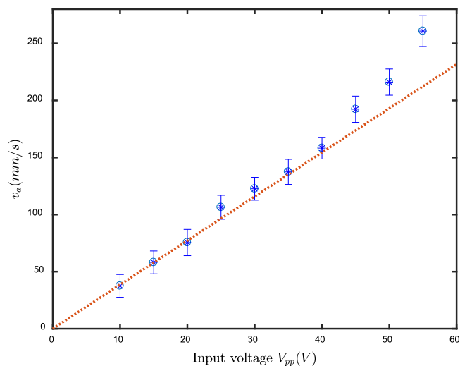
Fig. 2. Acoustic vibration amplitude varies with input voltage.
