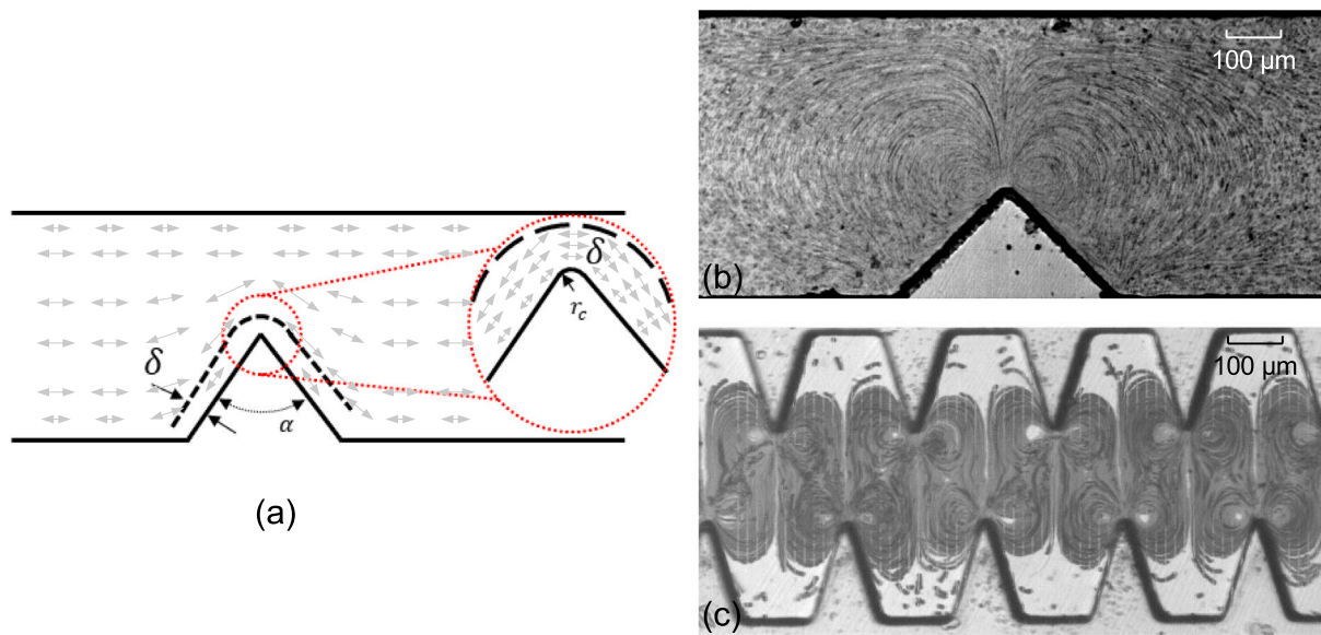
Fig. 3. Origin of the acoustic streaming around the sharp edge. (a) Sharp edge of angle \alpha and curvature diameter 2r_c inside a channel, \delta shows the boundary layer thickness; Gray arrows represent acoustic oscillations driven by piezoelectric transducer. Particle visualization of (b) single sharp-edge and (c) multiple sharp-edges acoustic streaming.
