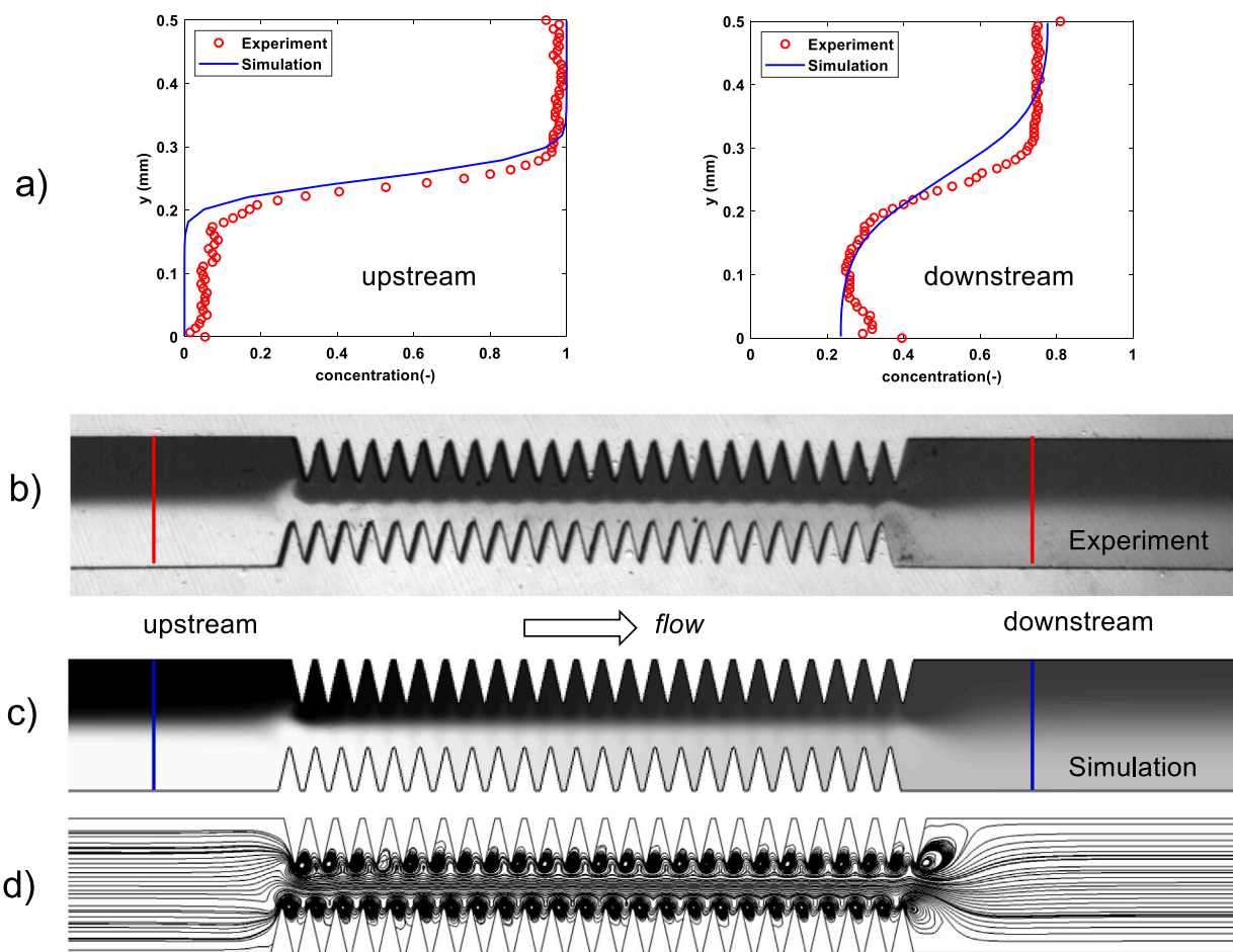
Fig. 5. Experimental validation of numerical results on active acoustic streaming driven mixing of two miscible fluids (water, water with Methylene blue) using micromixer S1. (a) Concentration profiles before (upstream, left) and after (downstream, right) the SEAS mixing channel. The concentration profiles are taken at a distance of 0.5 mm before and after the first/last sharp edge, where the profiles are not perturbed by remaining vorticity, (b) Experimental concentration evolution in the mixing channel, (c) Same concentration field obtained numerically, (d) Flow streamlines obtained numerically. The acoustic amplitude is v_a=85 mm/s and the flow rate is Q_c=8 \mu L/min. Concentration is normalized according to gray-scale contrast between two inlet fluids, i.e., from 0 to 1.
