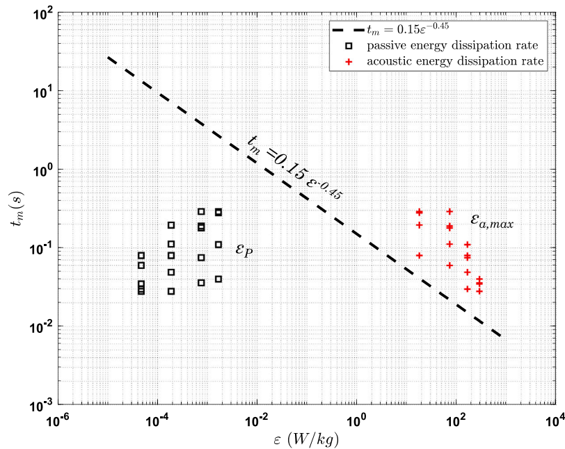
Fig. 11. Micromixing time t_m vs energy dissipation rates \epsilon .
