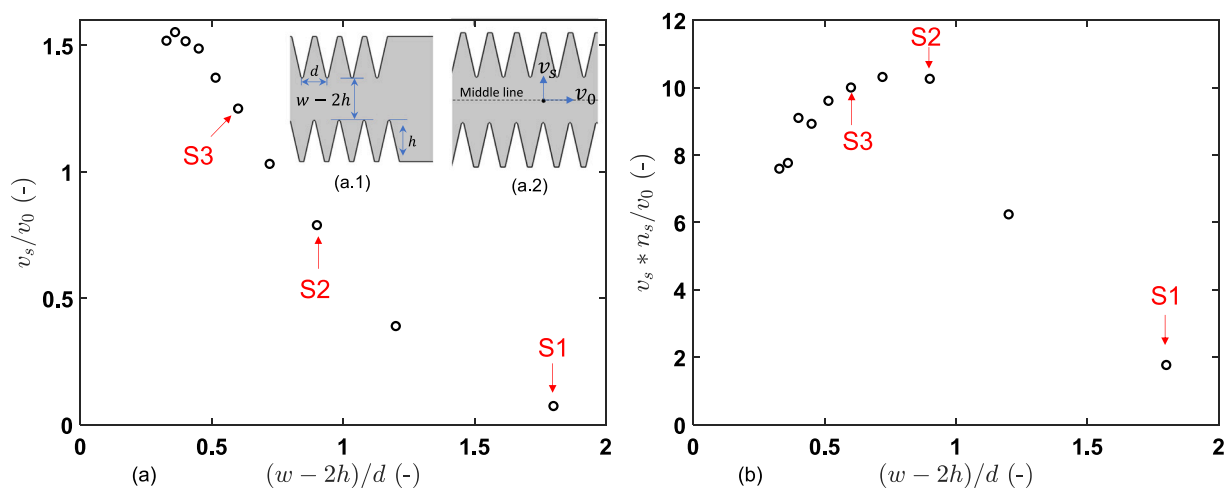
Fig. 7. Parametric simulation of mixing enhancement indicators by adjusting sharp edge patterns. Ratio v_s/v_0 versus (w-2h)/d for different sharp-edge micromixers (left). Quantity n_s \times v_s/v_0 versus (w-2h)/d , showing S2 as an optimal geometry for mixing (right). The sharp edge section ( l_2 ) is kept the same for the variety of edge densities.
