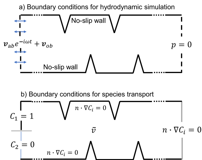
Fig. 4. Boundary conditions used in the DNS modeling.
