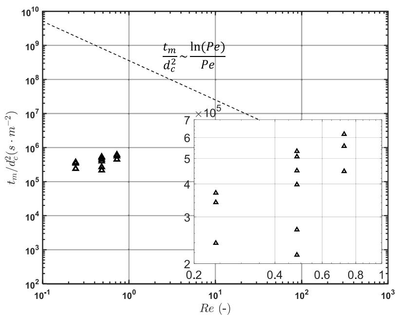
Fig. 10. Quantity t_m/d_c^2 versus channel Reynolds number.
